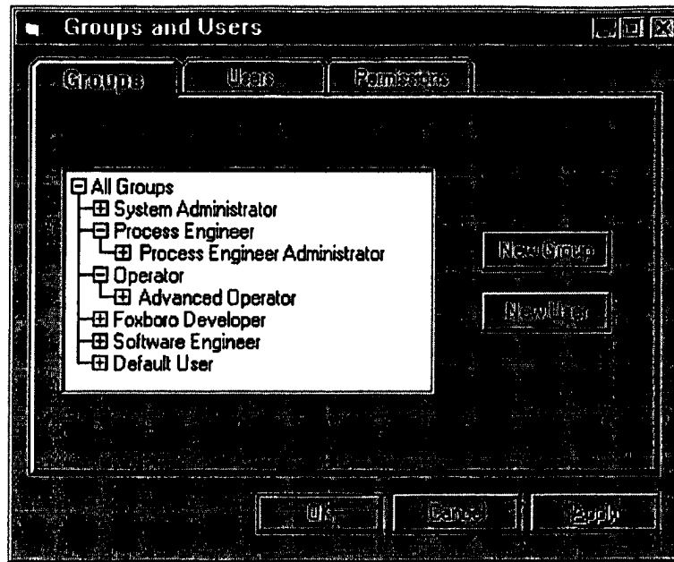
Figure 63 - Managing Groups
